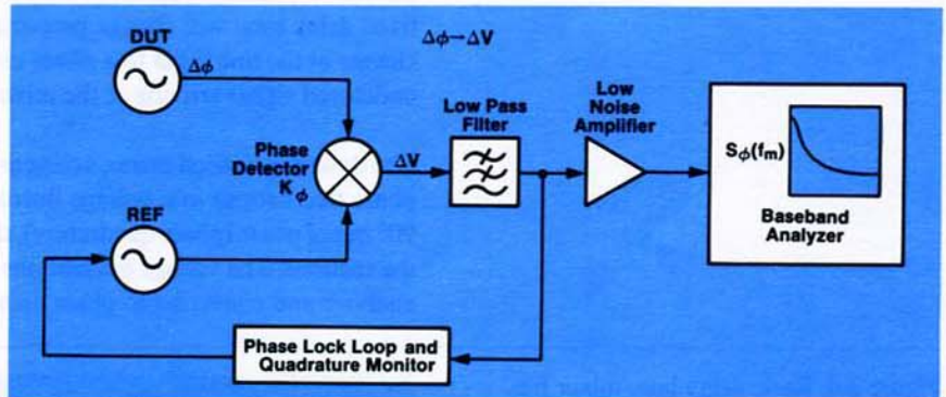
Figure 3.3. Basic phase detector method.
