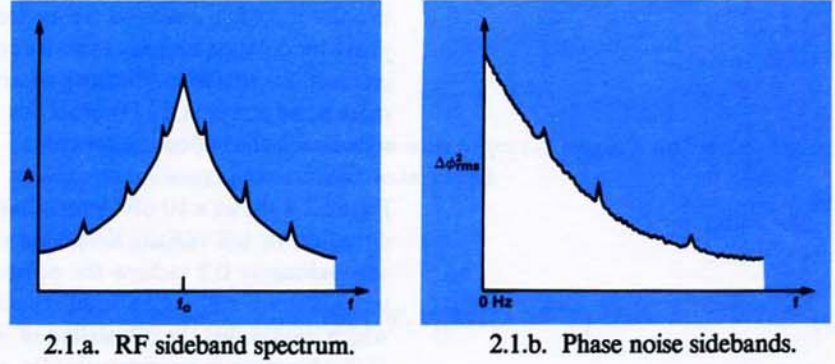
Figure 2.1. CW Signal sidebands viewed in the frequency domain.
