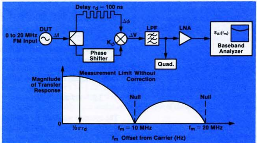
Figure 3.5. Nulls in sensitivity of delay line discriminator.
